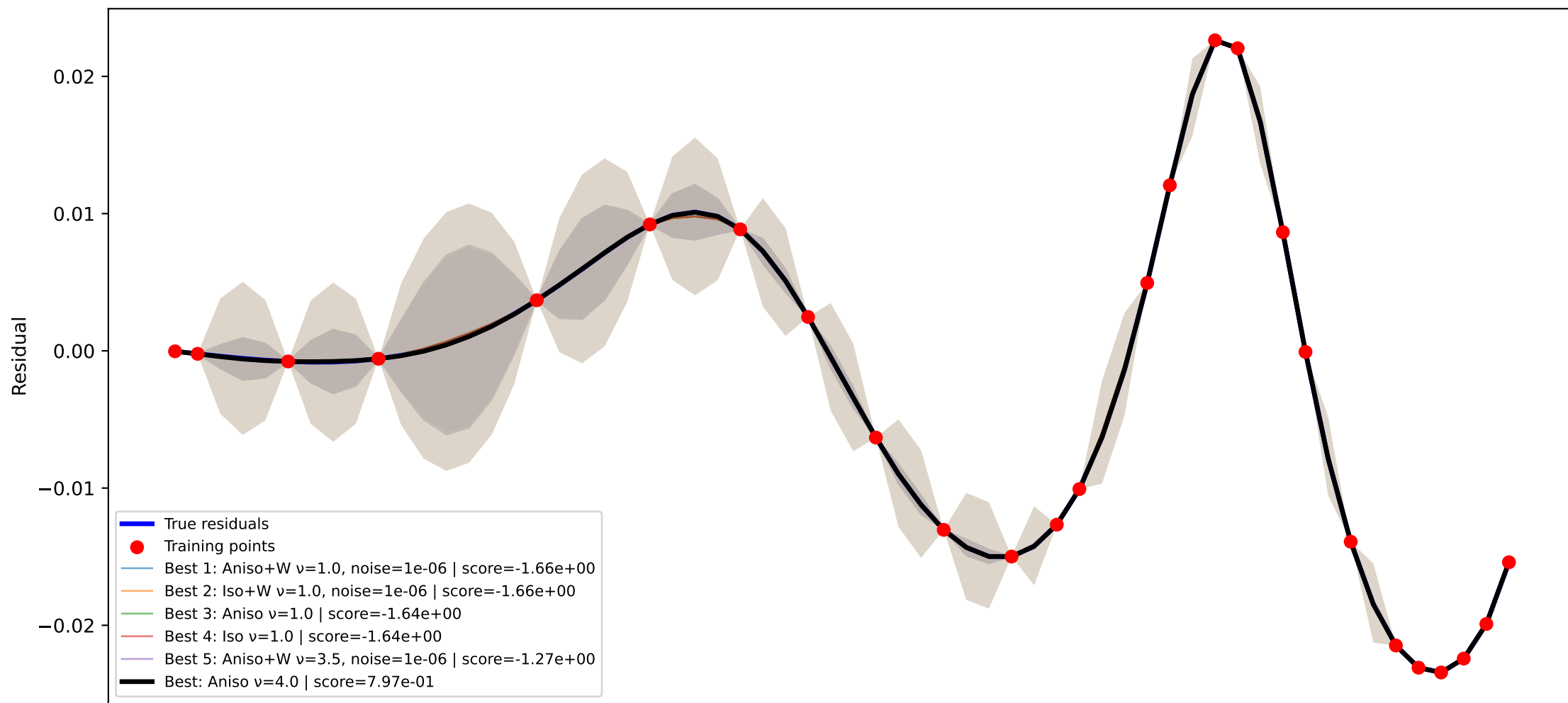
GPR kernel comparison node=10 RMSE=2.082e-05, train RMSE=8.230e-11
